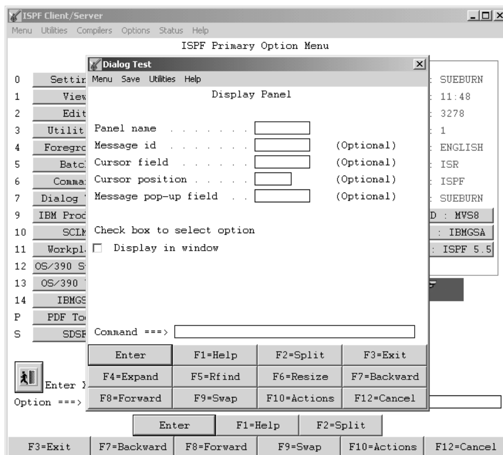
Figure 15. ISPF Dialog Test Display Panel Displayed Using ISPF Workstation Agent.
