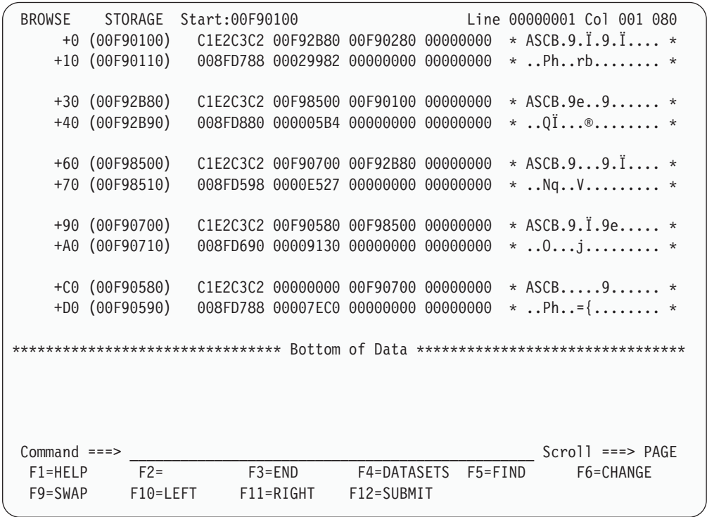
Figure 73. CHAIN Storage Format
