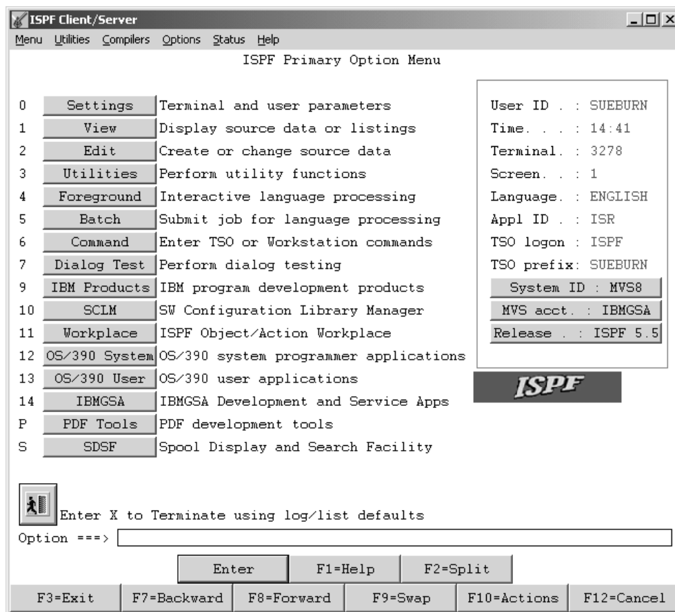
Figure 13. ISPF Primary Option Menu Displayed Using ISPF Workstation Agent
