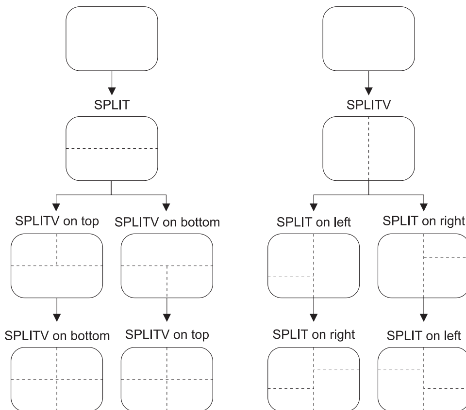
Figure 21. Splitting the 3290 Screen
