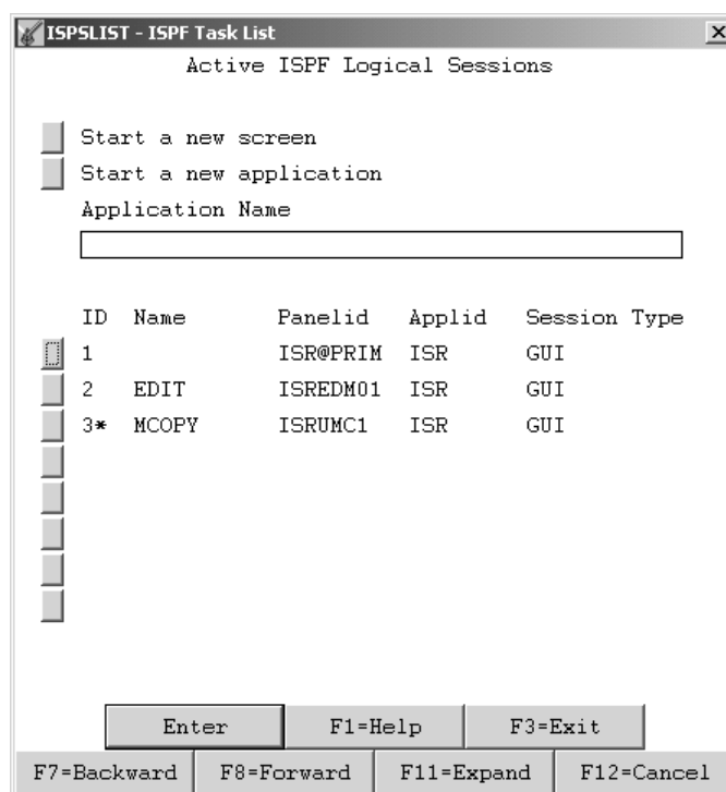
Figure 20. ISPF Task List
