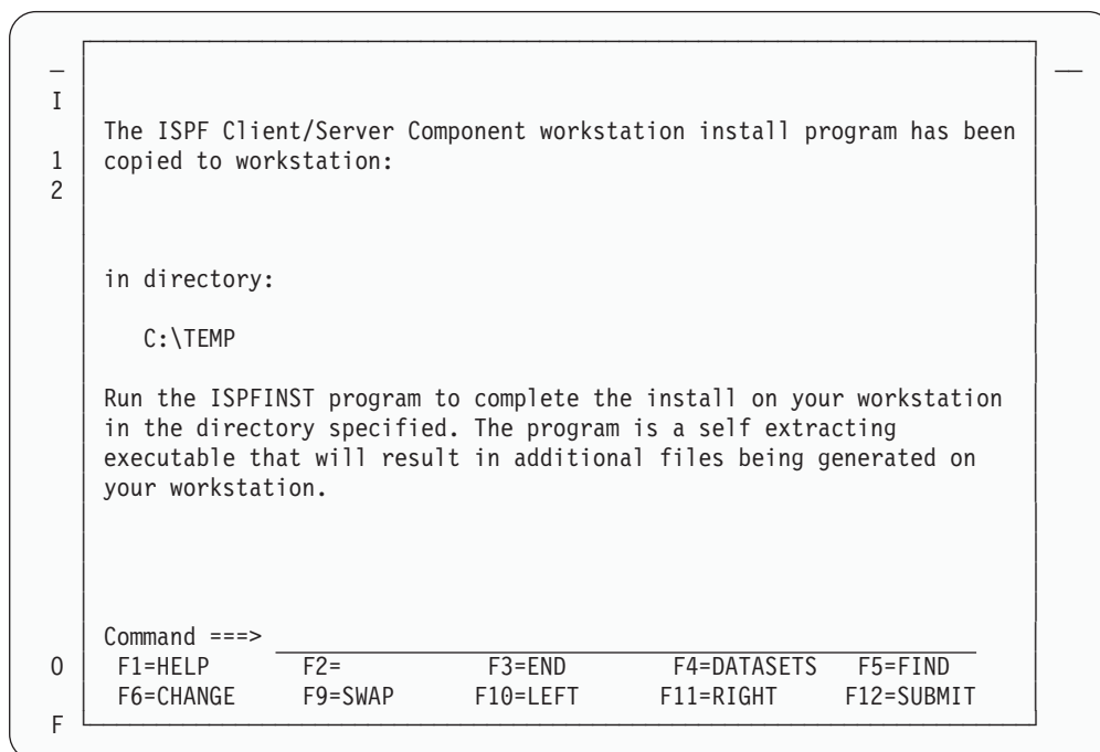
Figure 46. ISPF Client/Server Component Install Program Panel (ISPWSD07)
