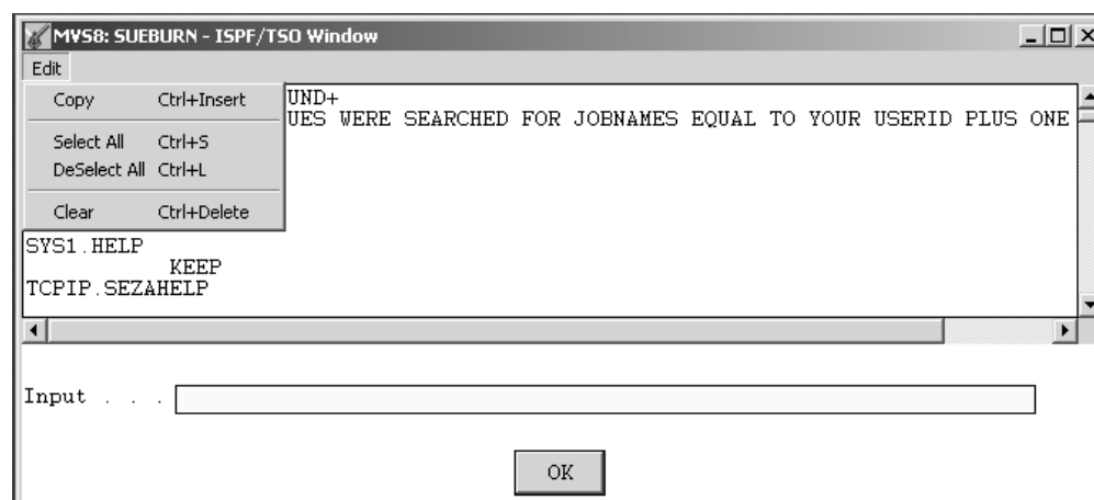
Figure 19. ISPF/TSO GUI Window with Pull-Down Menu
