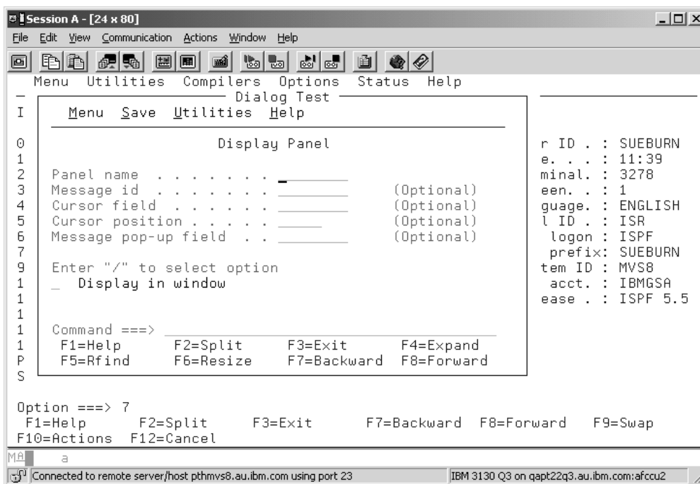
Figure 14. ISPF Dialog Test Display Panel Displayed on a 3270 Emulator
